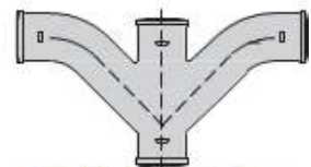
Double Combination Wye & 1/8" Bend
